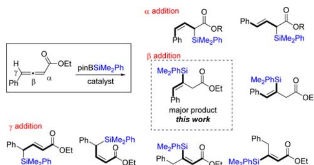
Scheme 1. Possible Silylation Products
